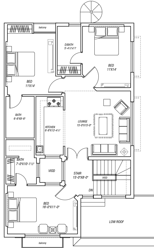
1st FLOOR PLANS
