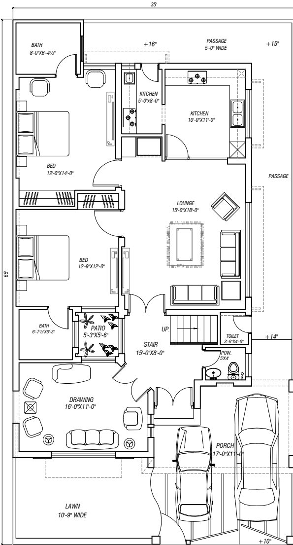
GROUND FLOOR PLANS
