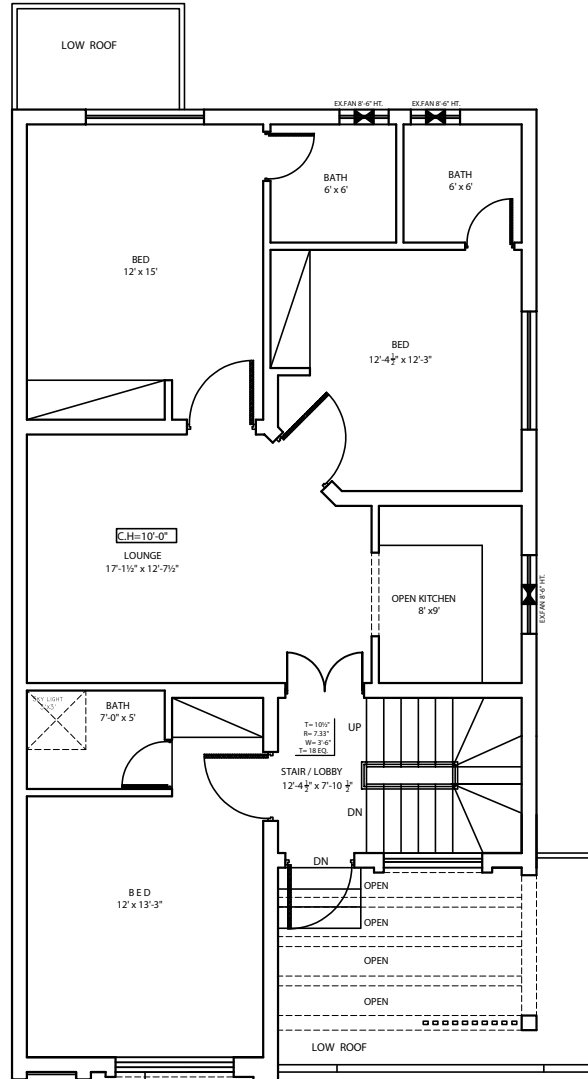
1st FLOOR PLANS
