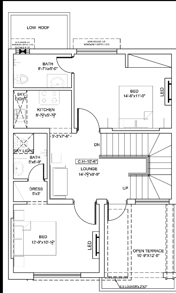
1st FLOOR PLANS
