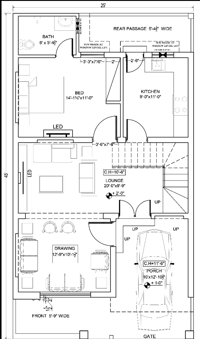
GROUND FLOOR PLANS
