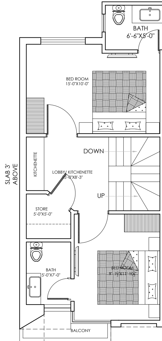
1st FLOOR PLANS
